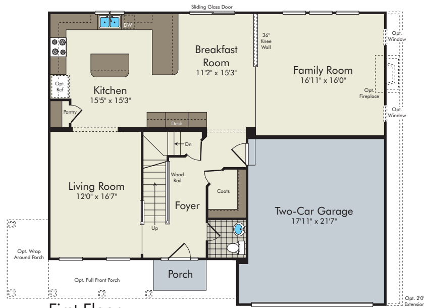
First Floor w/ Alternate Kitchen & 20' Rear Extension
